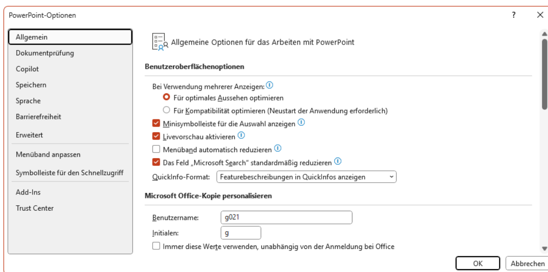
Abb. 1: Dialogfeld PowerPoint-Optionen
